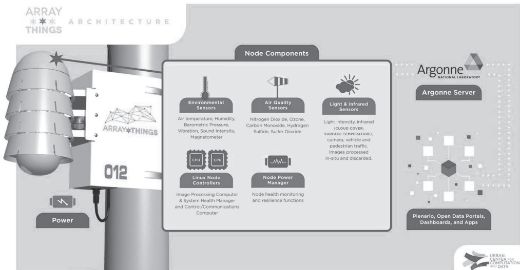
Figure 2: Architecture of the Array of Things system [1]
